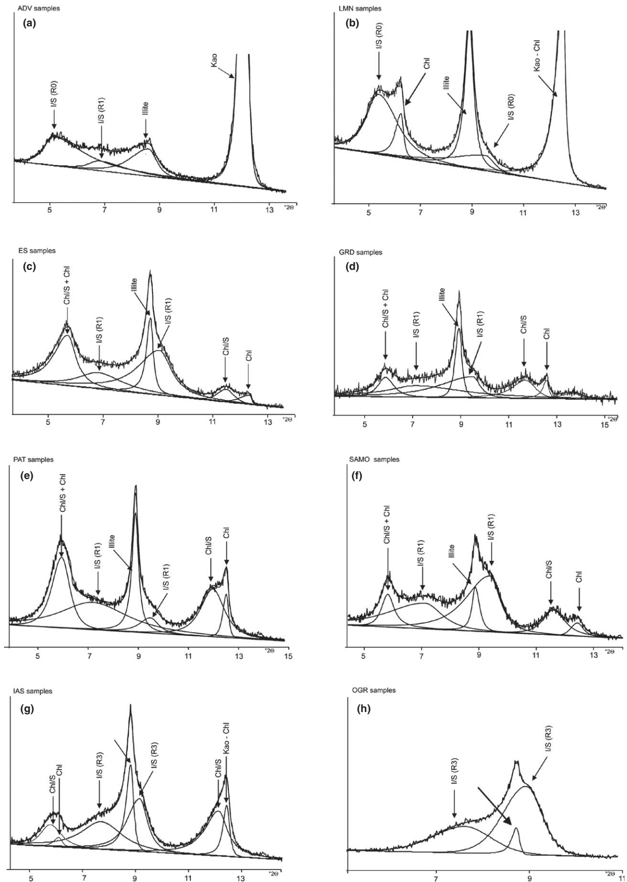
Fig. 6. Decomposition at low angles of the characteristic diffraction profile of ADV, LMN, ES, GRD, PAT, SAMO, IAS and OGR samples ( <2 \mu\text{m} fraction).
