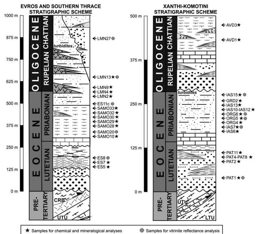
Fig. 3. Synthetic and schematic stratigraphic sections with location of the studied samples (modified from Caracciolo et al. , 2011a). CRB, Circum-Rhodope Belt; UTU, Upper Tectonic Unit; LTU, Lower Tectonic Unit. The 'Evros and southern Thrace stratigraphic scheme' is located in the Evros depocentre (see Fig. 1) and the 'Xanthi-Komotini stratigraphic scheme' is located in the Xanthi-Komotini depocentre (see Fig. 1).
