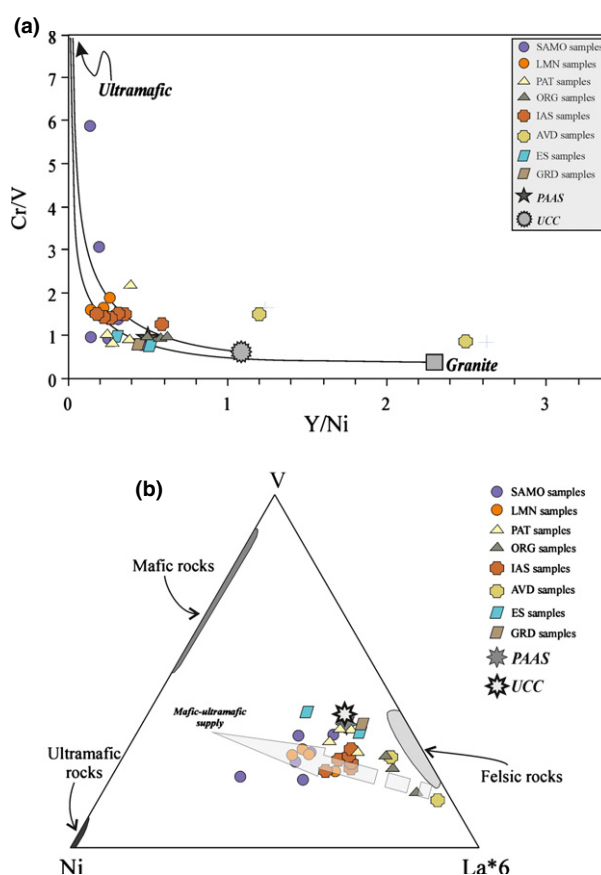
Fig. 8. (a) Analyzing the provenance by using relations of Cr/V vs Y/Ni. Curve model mixing between granite and ultramafic end-members. (b) V-Ni-La*6 ternary diagram, showing fields representative of felsic, mafic and ultramafic rocks plot separately (modified from Perri et al. , 2011b).
