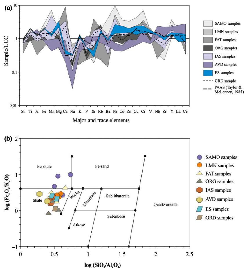
Fig. 5. (a) Normalization of major and trace elements to upper continental crust averages (after McLennan et al. , 2006). The plot of the Post-Archaean Australian Shales (PAAS; Taylor & McLennan, 1985) is shown for comparison. (b) Classification diagram for the studied samples (after Herron, 1988).
