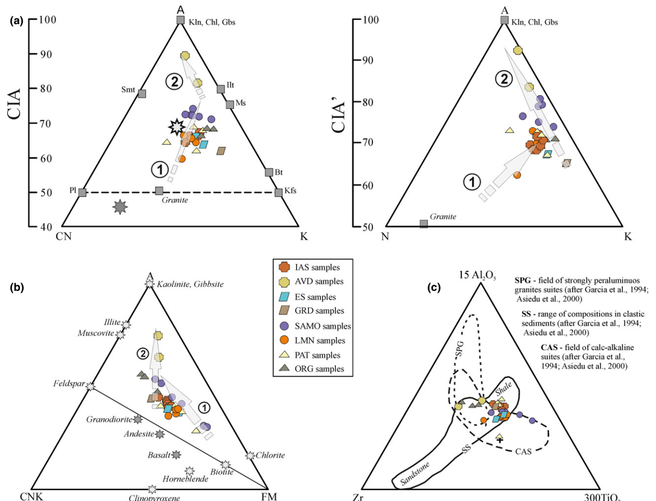
Fig. 9. (a) Ternary A-CN-K and A-N-K diagrams. Legend: Ms, muscovite; Illt, illite; Kln, kaolinite; Chl, chlorite; Gbs, gibbsite; Smt, smectite; Bt, biotite; Kfs, K-feldspar; Pl, plagioclase; A, Al 2 O 3 ; CN, CaO + Na 2 O; K, K 2 O; CIA, Chemical Index of Alteration (modified from Nesbitt & Young, 1982). (b) A-CN-K-FM ternary diagram of the studied samples. A, Al 2 O 3 ; CNK, CaO + Na 2 O + K 2 O; FM, Fe 2 O 3 + MgO. (c) Ternary 15Al 2 O 3 -300TiO 2 -Zr plot after García et al. (1994), suggesting poor sorting and rapid deposition of the sediments.
