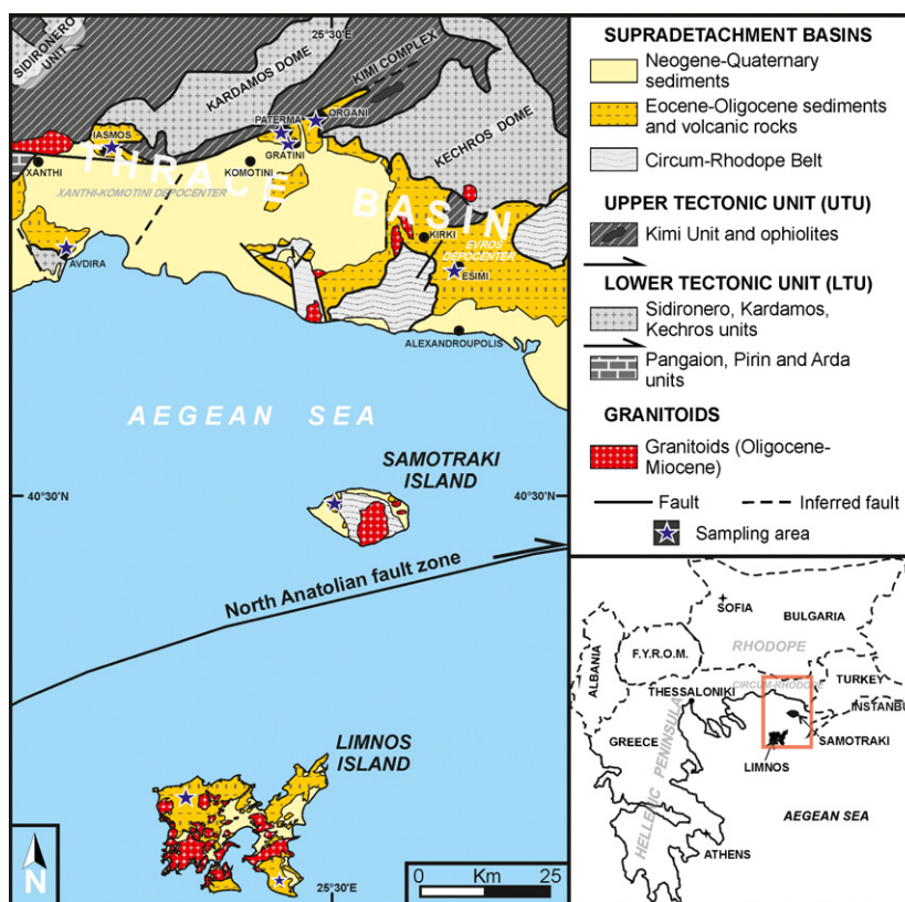
Fig. 2. Simplified geological map of the Rhodope province with the location of the studied samples. The Thrace Basin and the other structural units are shown (modified after Kiliyas et al. , 2011a,b).
