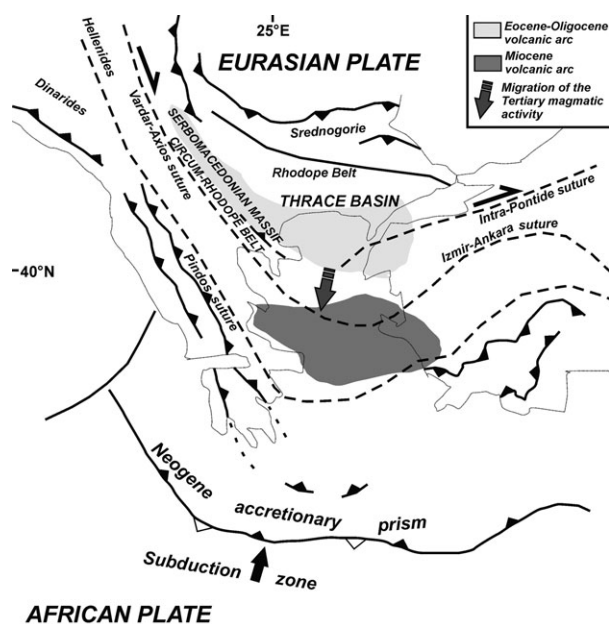
Fig. 1. Schematic sketch with the position of the Thrace Basin with respect to the main tectonic units and structures of the eastern Mediterranean region (modified after Kilias et al. , 2011a,b).
