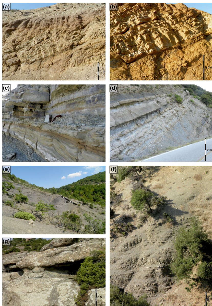
Fig. 4. Exposure of key lithofacies of the stratigraphic sections where the studied samples have been collected. (a) Samotraky section characterized by graded sandstones alternating with mudrocks. (b) Particular of Samotraky section with 10–50 cm sandstone beds alternating with fine mudrocks. (c) Limnos section characterized by medium to fine-grained stratified sandstones alternating with mudrocks; the lower portion shows soft-sediment deformation structures. (d) Section between Paterma and Organi villages characterized by centimetre-to-metre-thick graded sandstones alternating with siltstones and mudrocks. (e) Section between Paterma and Gratini villages characterized by metre-thick stratified siltstones and mudrocks alternating with thin-bedded fine to medium-grained sandstones. (f) View of the passage from mudrocks and siltstones alternating with centimetre-thick fine-grained sandstones to metre-thick mudrocks and siltstones of the Iasmos section. (g) Coarse-grained sandstone and gravel beds alternating with mudrocks of the Esimi section.
