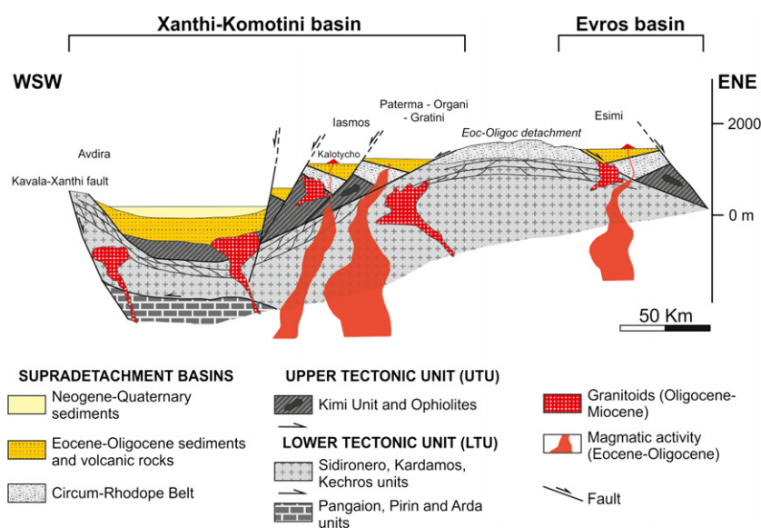
Fig. 10. Schematic sketch of the fault geometry and kinematics and magmatic activity during Paleogene-Neogene extension of Rhodope Massif (modified after Kiliyas et al. , 2011a,b), referred to the Figs 1 and 2.
